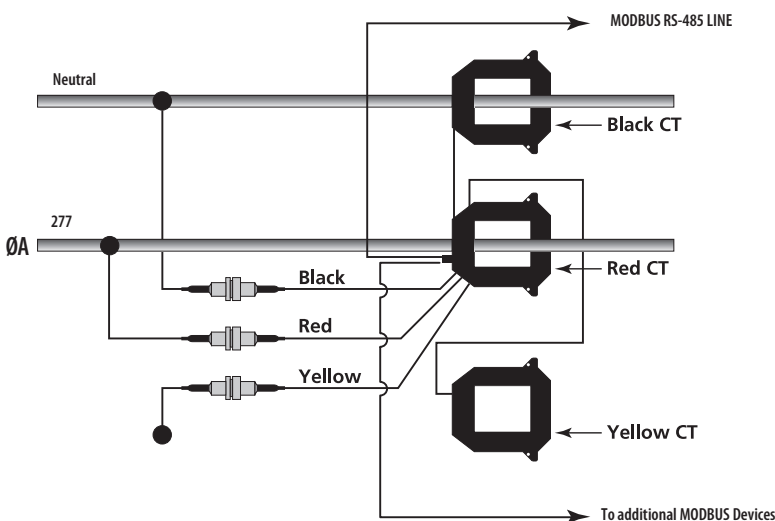
Typical 277 VAC 1Ø, 2-Wire Installation
