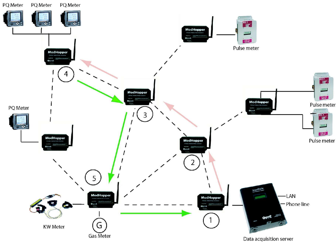
Figure 3 – Return path for data request
