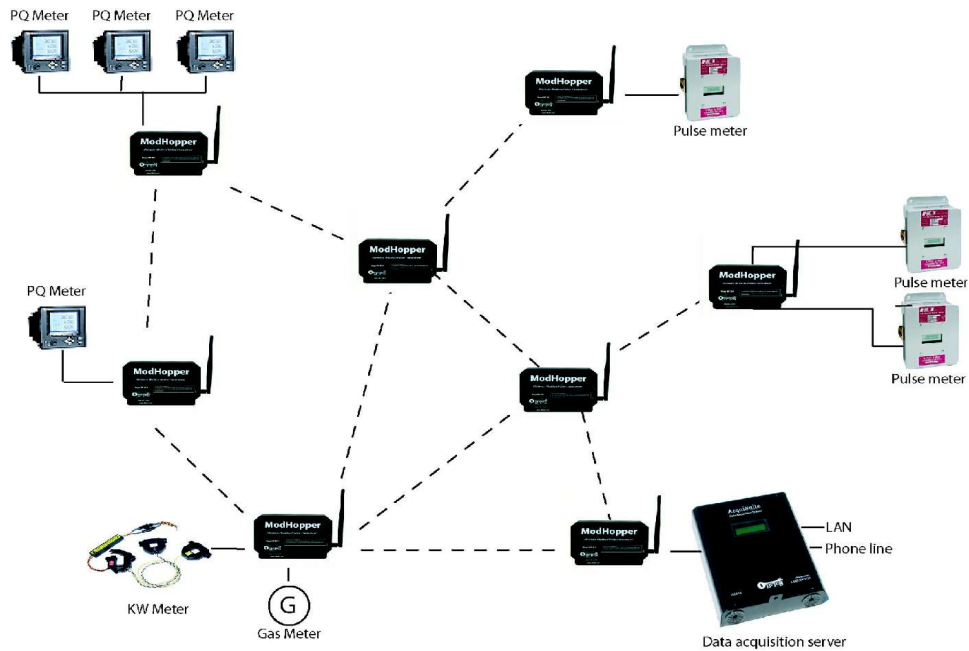
Figure 1 – Mesh network topology
