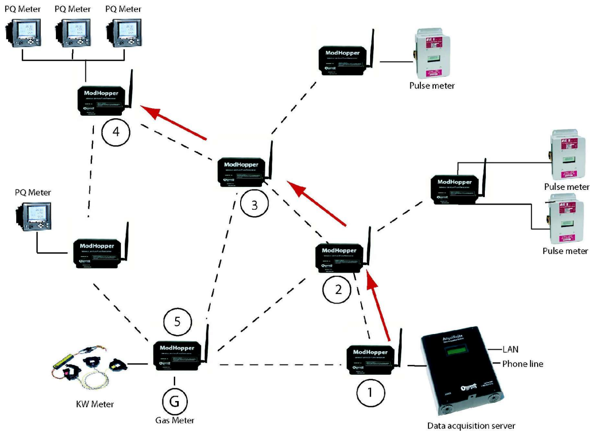
Figure 2 – Modbus request path
